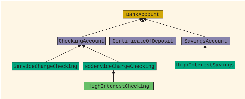
FIGURE 10-7 Inheritance hierarchy of bank accounts
