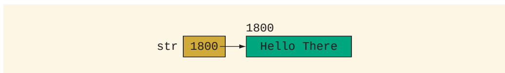
FIGURE 7-8 str after the statement str = "Hello There"; or str = str + " There"; executes
