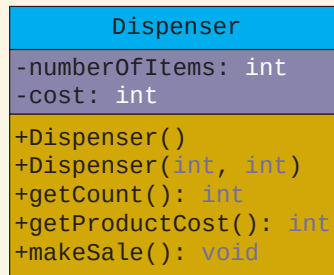
FIGURE 8-20 UML class diagram of the class Dispenser
