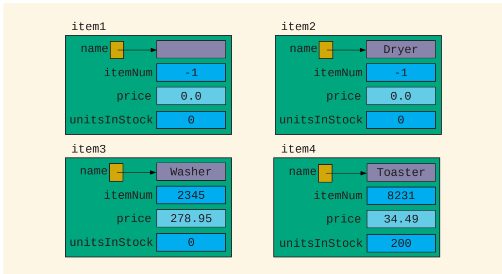
FIGURE 8-14 Effect of constructors on objects
