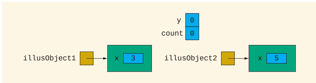
FIGURE 8-15 illusObject1 and illusObject2
