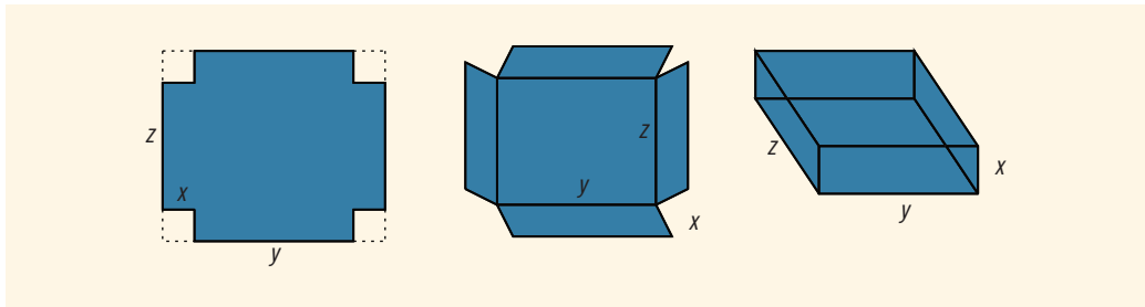
FIGURE 7-17 Cardboard box
