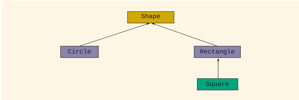
FIGURE 10-1 Inheritance hierarchy
