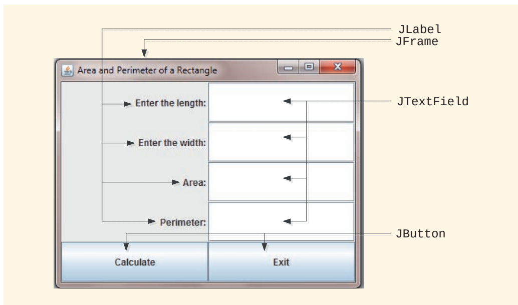
FIGURE 6-3 Java GUI components
