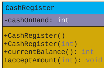
FIGURE 8-19 UML class diagram of the class CashRegister
