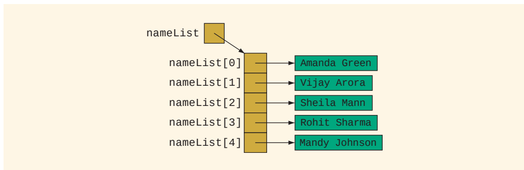
FIGURE 9-11 Array nameList
