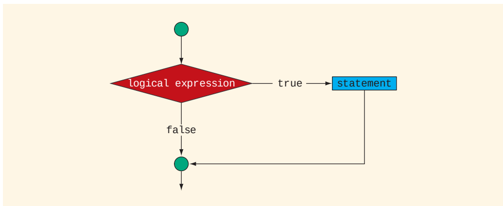
FIGURE 4-2 One-way selection
