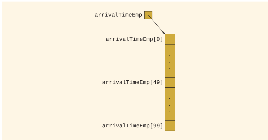
FIGURE 9-12 Array arrivalTimeEmp
