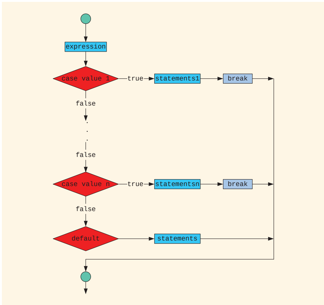
FIGURE 4-5 switch statement
