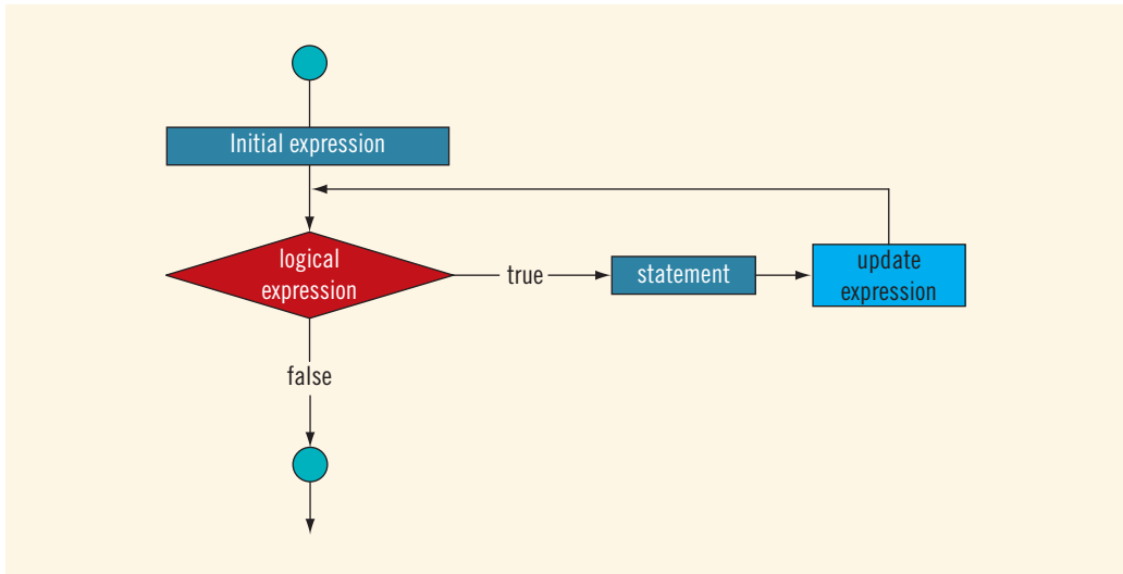
FIGURE 5-4 for loop
