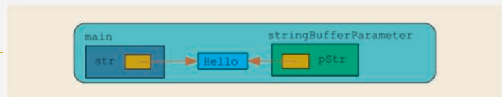
FIGURE 7-14 Variable before the statement in Line 7 executes
