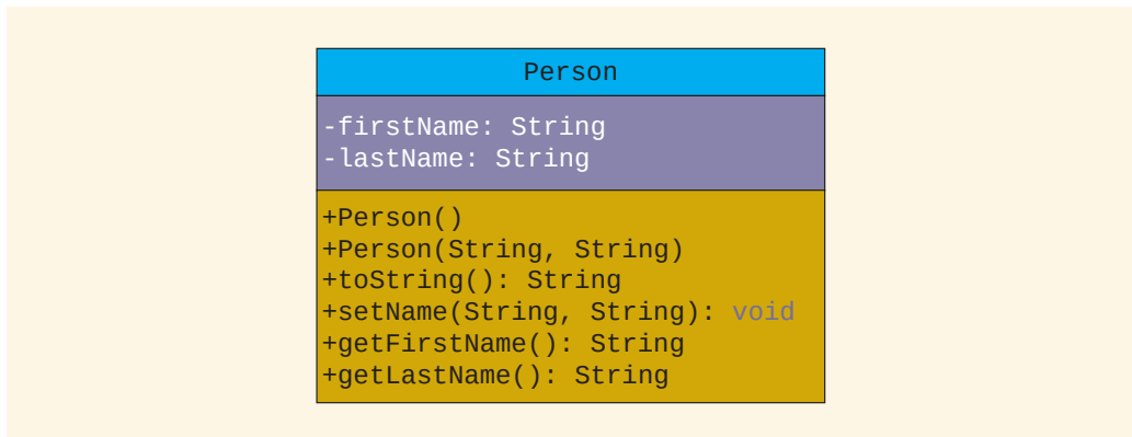
FIGURE 8-18 UML class diagram of the class Person
