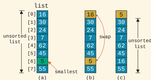
FIGURE 14-3 Elements of list during the first iteration
