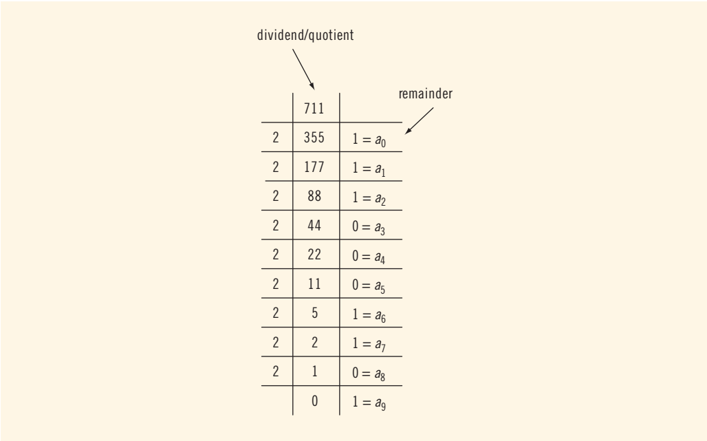
FIGURE D-2 Determining the binary representation of 711
