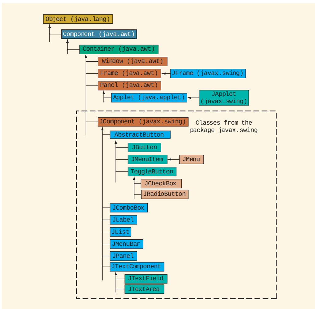
FIGURE 12-1 Inheritance hierarchy of GUI classes (classes shown in the dotted rectangle are from the package javax.swing )
