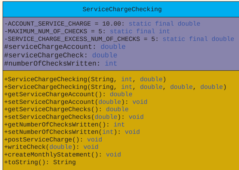
FIGURE 10-10 UML class diagram of the class ServiceChargeChecking
