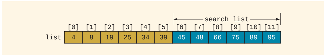
FIGURE 14-14 Search list, list[6]...list[11]
