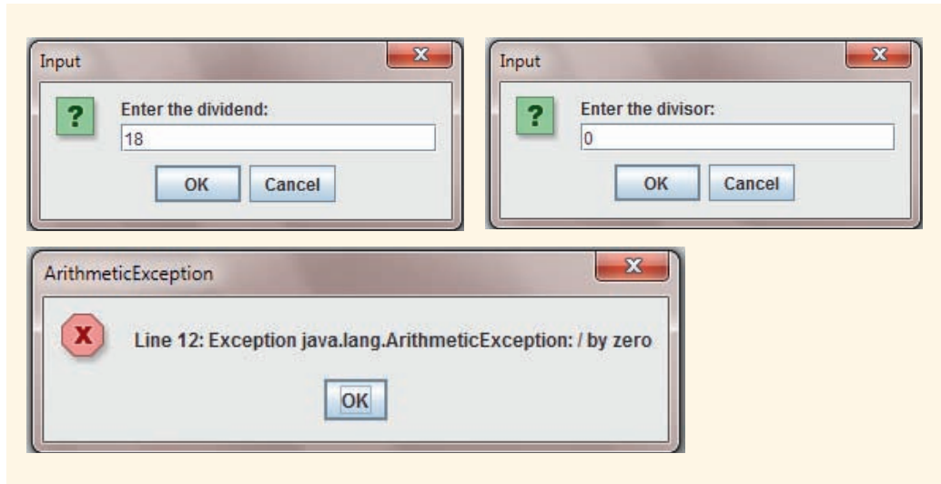
FIGURE 11-6 Sample Run 2 of the program ExceptionExample4
