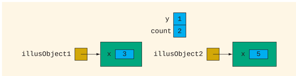
FIGURE 8-17 illusObject1 and illusObject2 after the statement Illustrate.count++ ; executes
