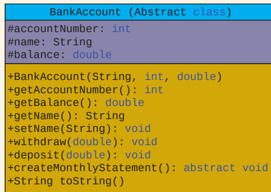
FIGURE 10-8 UML class diagram of the class BankAccount
