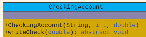
FIGURE 10-9 UML class diagram of the class CheckingAccount
