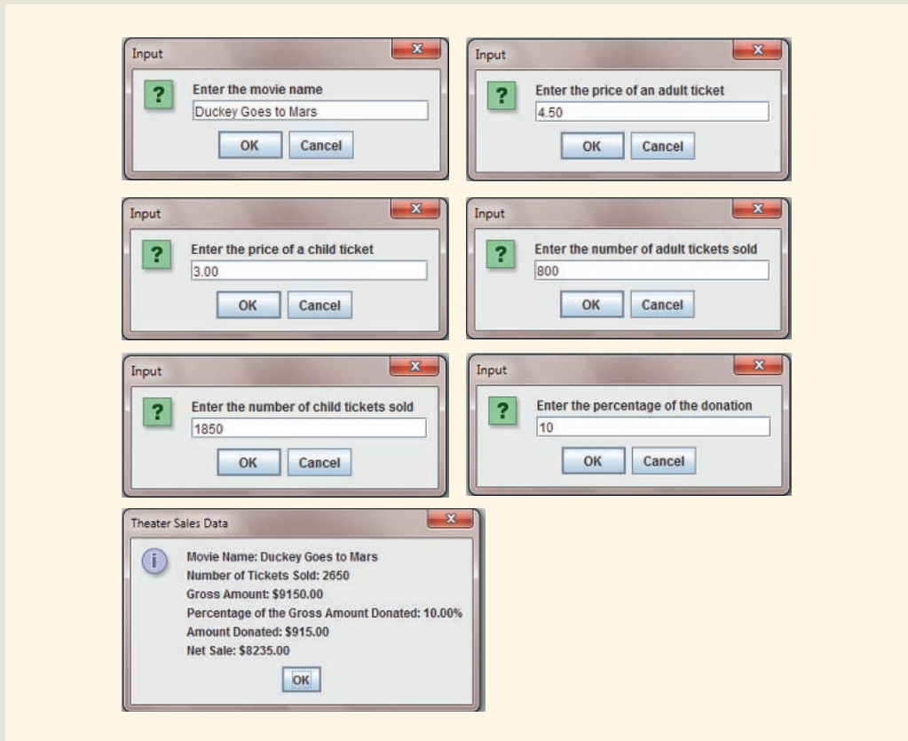
FIGURE 3-15 Sample run of movie sales program
