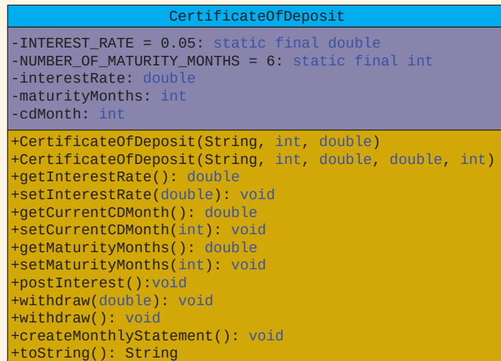
FIGURE 10-15 UML class diagram of the class CertificateOfDeposit
