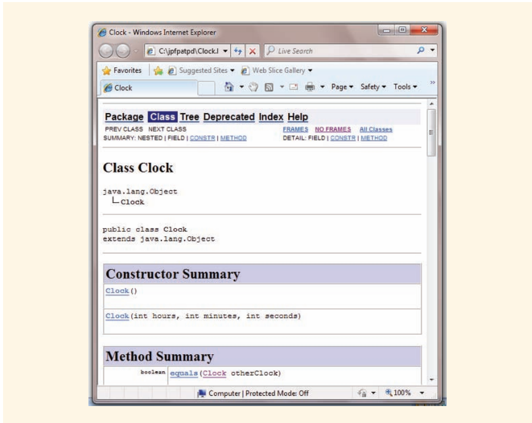
FIGURE D-20 Java style documentation of the class Clock
