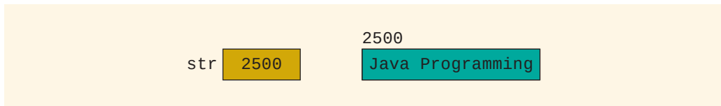
FIGURE 3-2 Variable str and the data it points to
