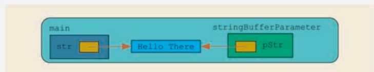
FIGURE 7-15 Variable after the statement in Line 14 executes
