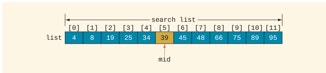
FIGURE 14-13 Search list, list[0]...list[11]
