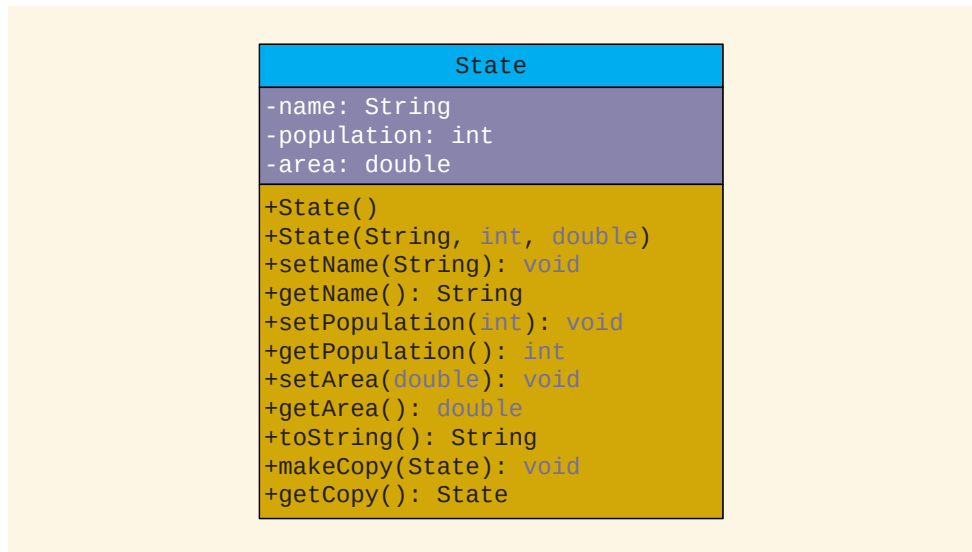
FIGURE 8-25 UML diagram
