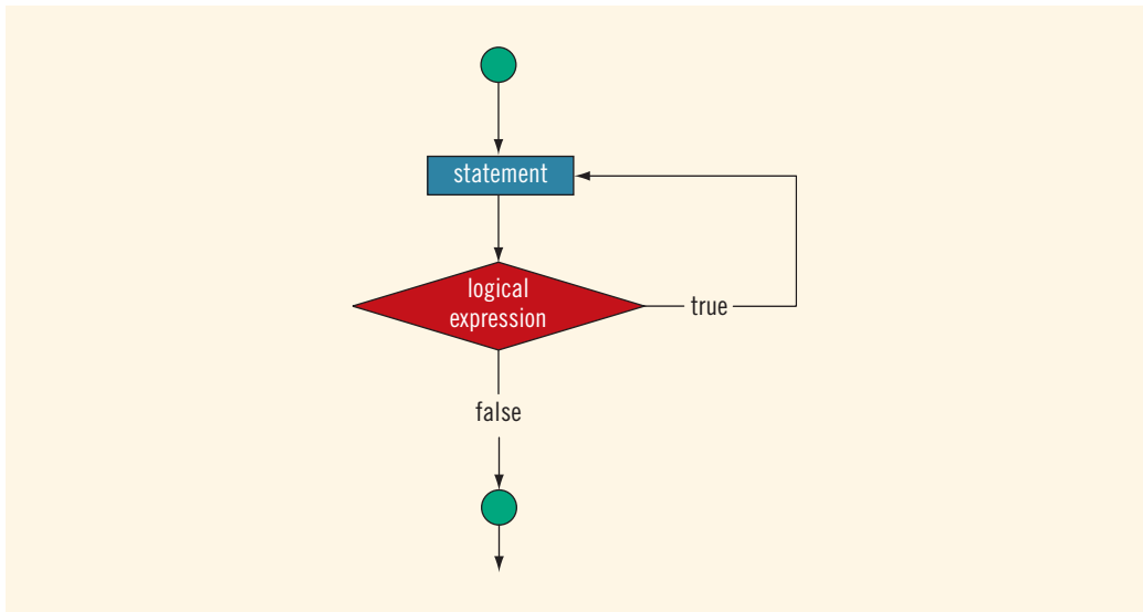
FIGURE 5-5 do...while loop
