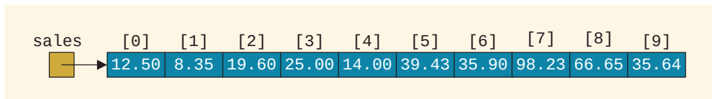
FIGURE 9-6 Array sales
