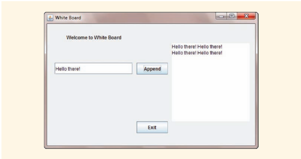
FIGURE 12-9 White Board GUI
