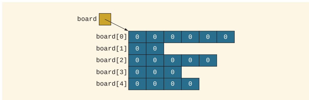
FIGURE 9-18 Array board
