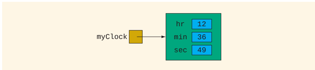
FIGURE 8-7 Object myClock
