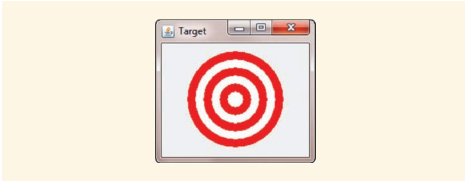
FIGURE 12-30 Target practice
