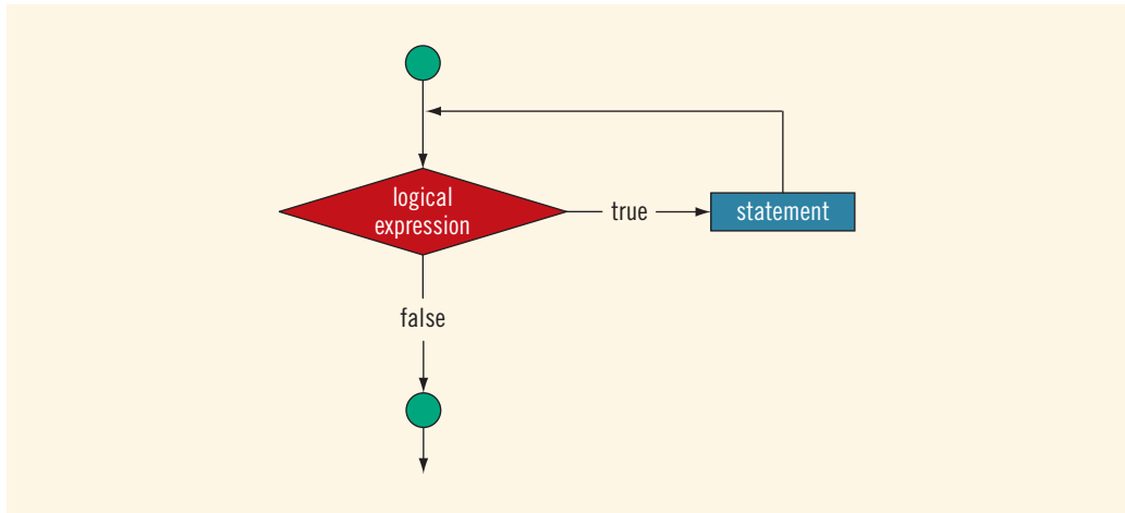
FIGURE 5-1 while loop
