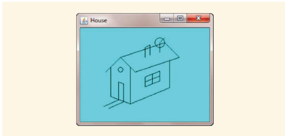
FIGURE 12-31 House
