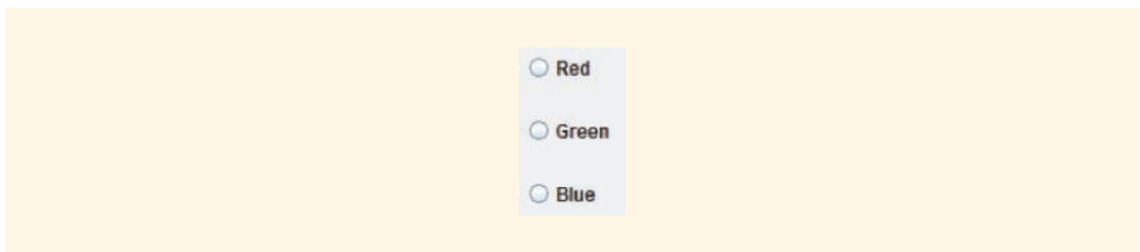
FIGURE 12-14 Radio buttons
