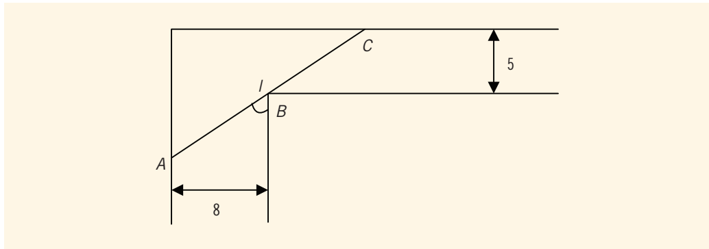
FIGURE 7-19 Pipe problem
