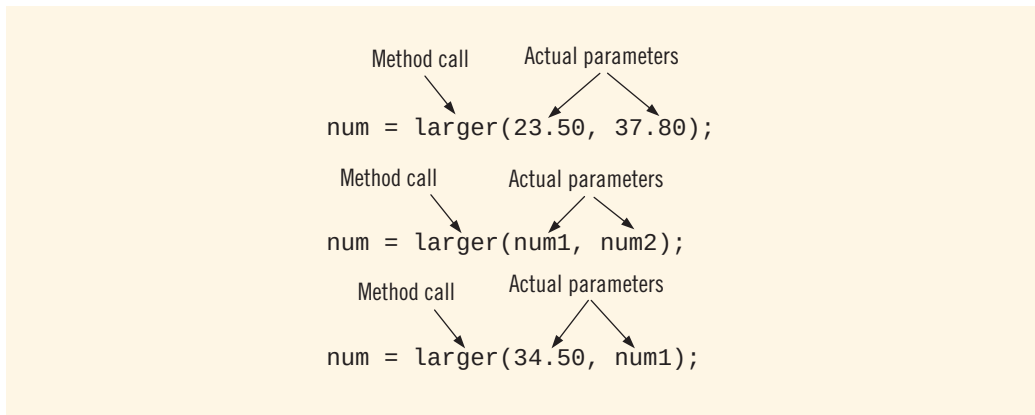
FIGURE 7-2 Method calls
