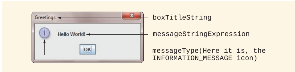
FIGURE 3-9 Message dialog box showing its various components
