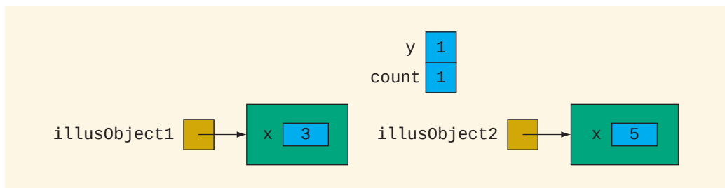
FIGURE 8-16 illusObject1 and illusObject2 after the statements Illustrate.incrementY(); and Illustrate.count++; execute
