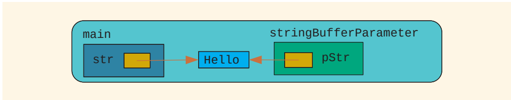
FIGURE 7-14 Variable before the statement in Line 7 executes
