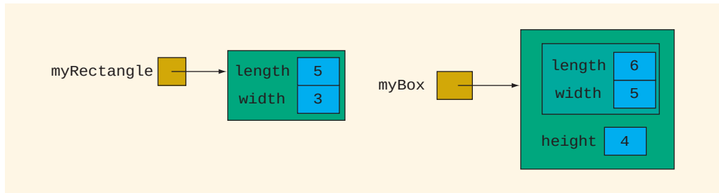
FIGURE 10-4 Objects myRectangle and myBox
