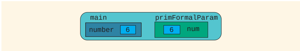
FIGURE 7-4 The variables number and num before execution of the statement in Line 13
